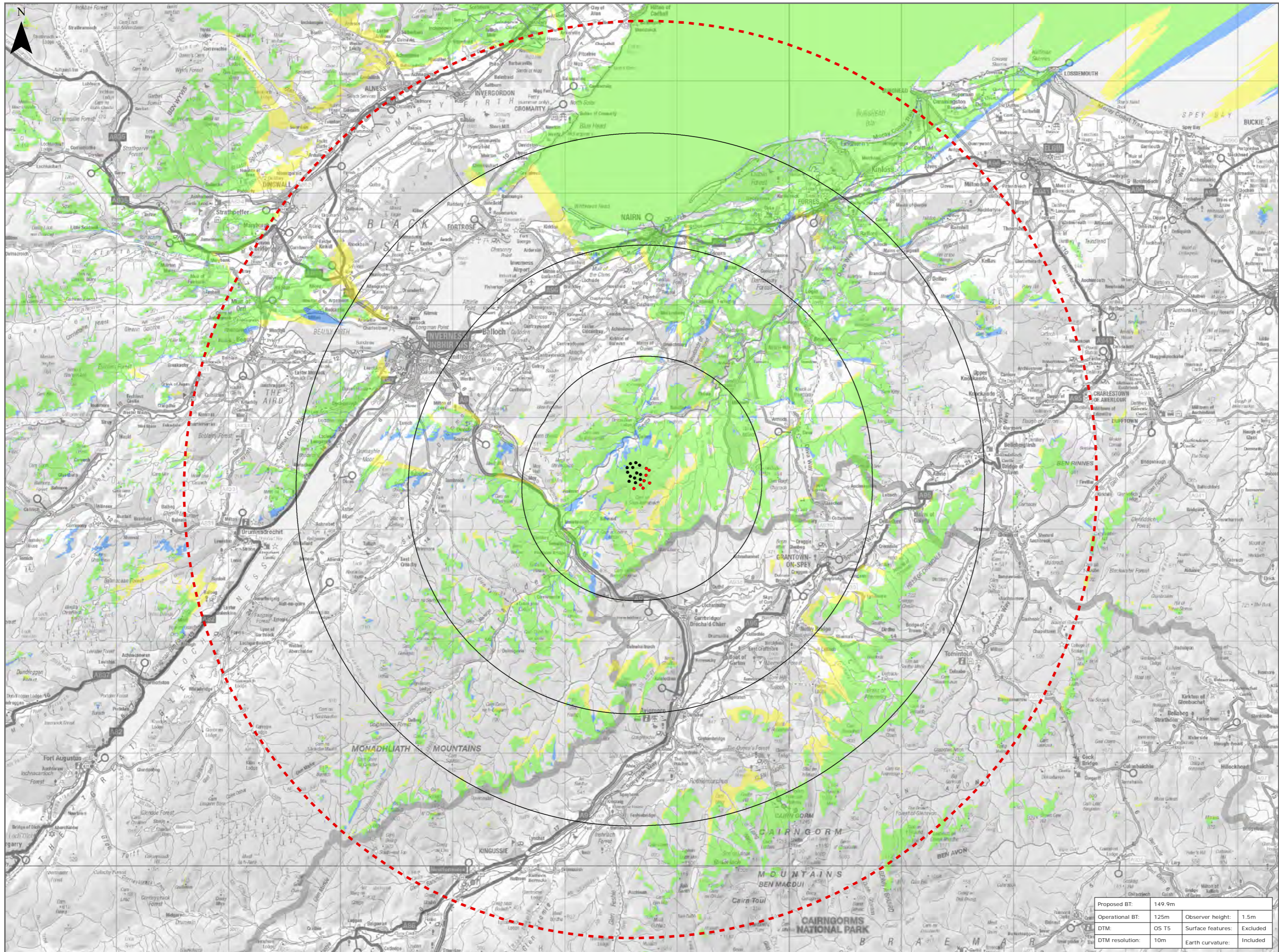
Figure 7.7: Comparative Blade Tip ZTV
