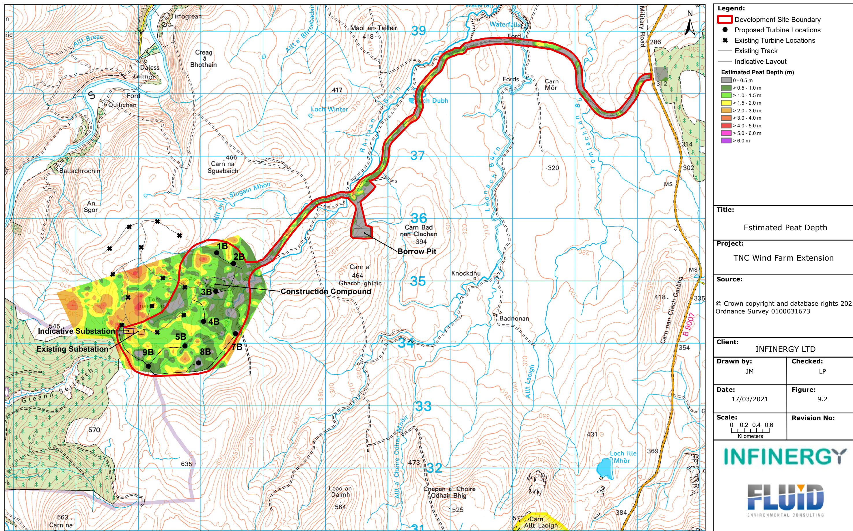
Figure 9.2: Estimated Peat Depth
