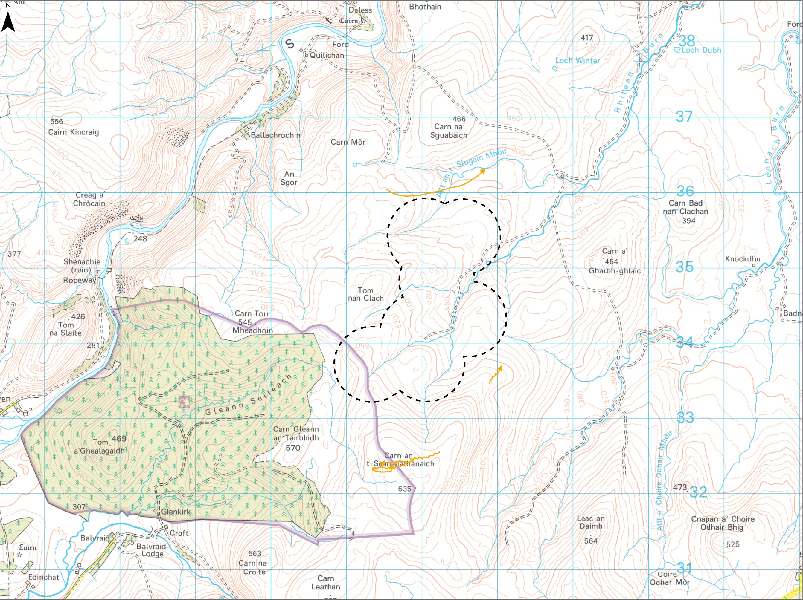
Figure 12.6: Golden eagle flights from GVPs
