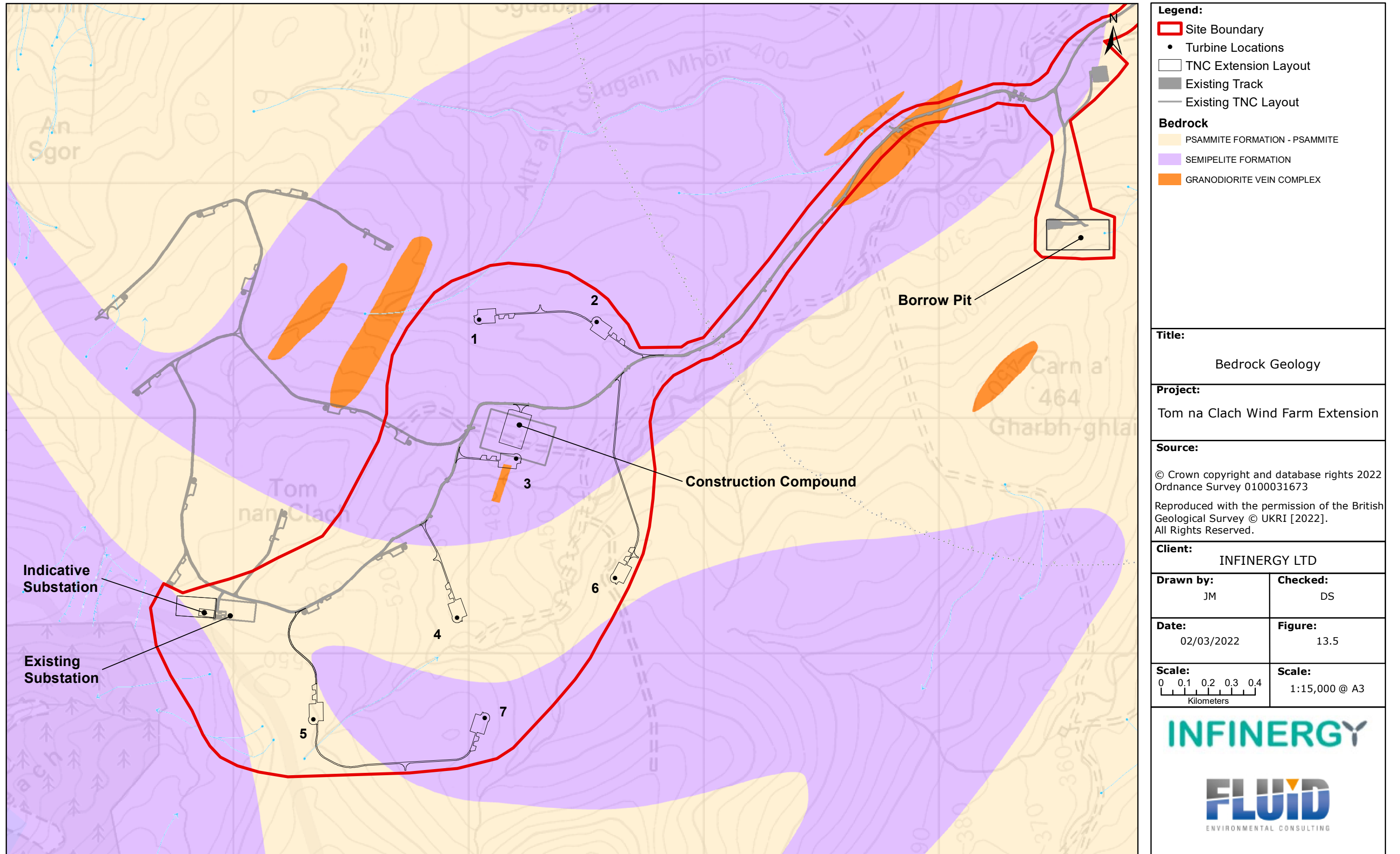
Figure 13.5: Bedrock Geology
