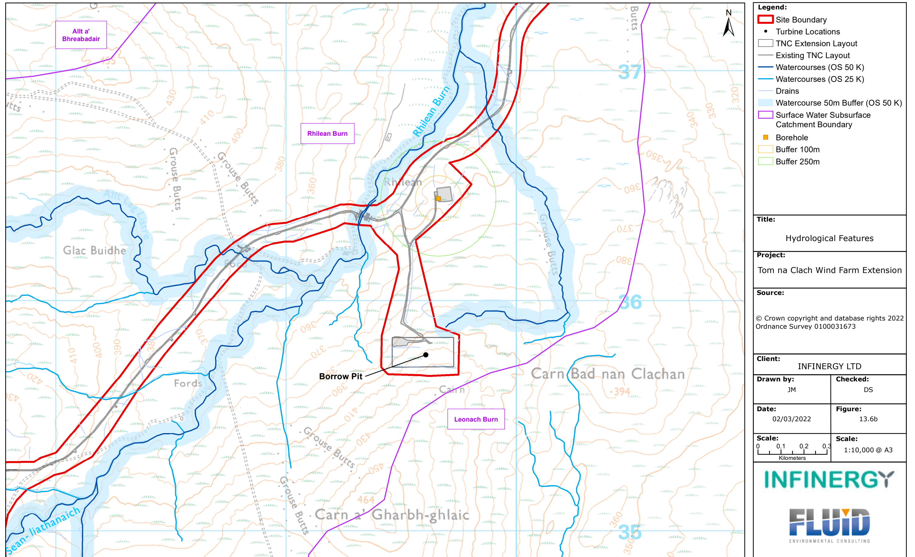
Figure 13.6b: Hydrological Features
