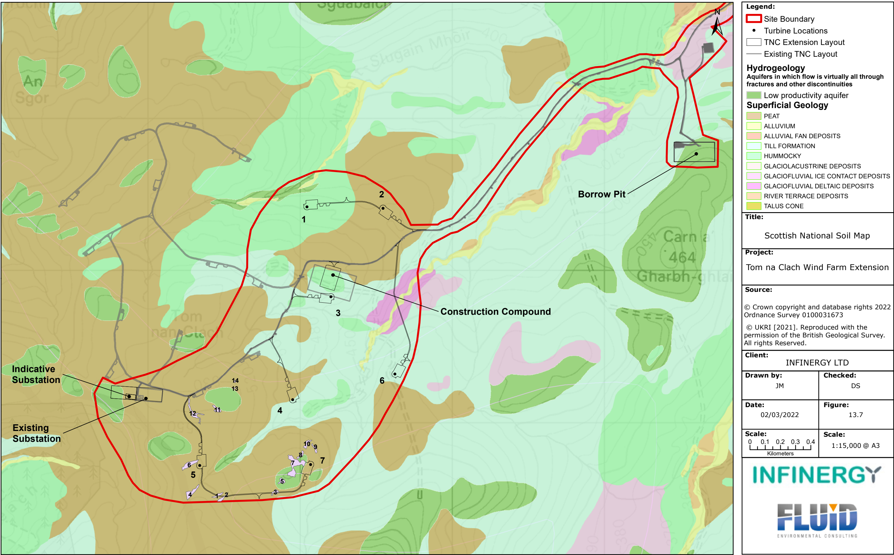
Figure 13.7: Hydrogeological Regime
