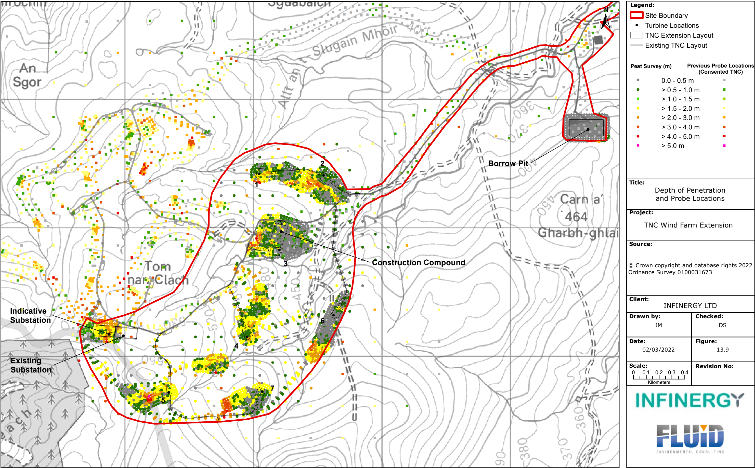
Figure 13.9: Depth of Penetration and Probe Locations
