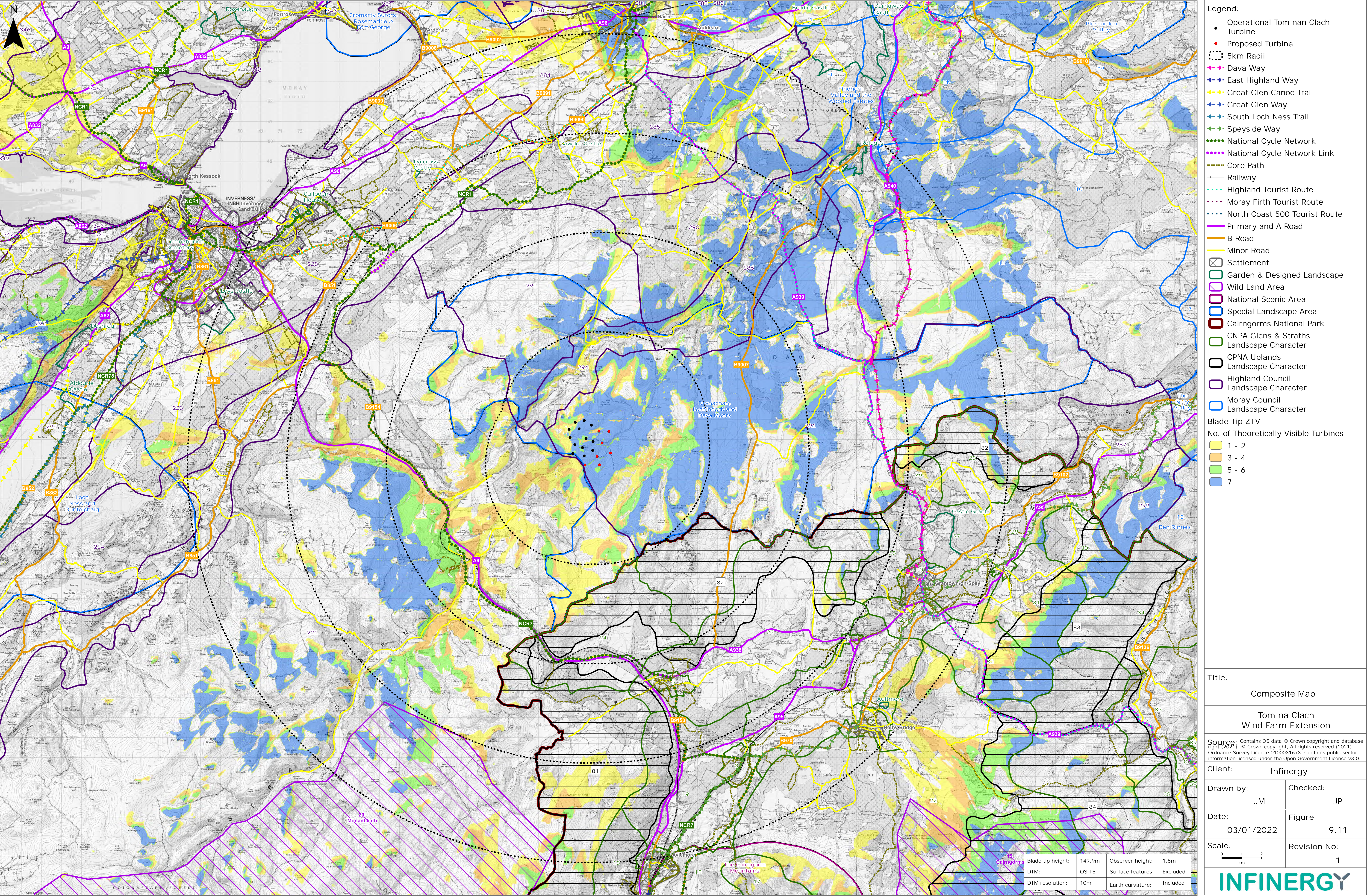
Figure 9.11 Composite Map
