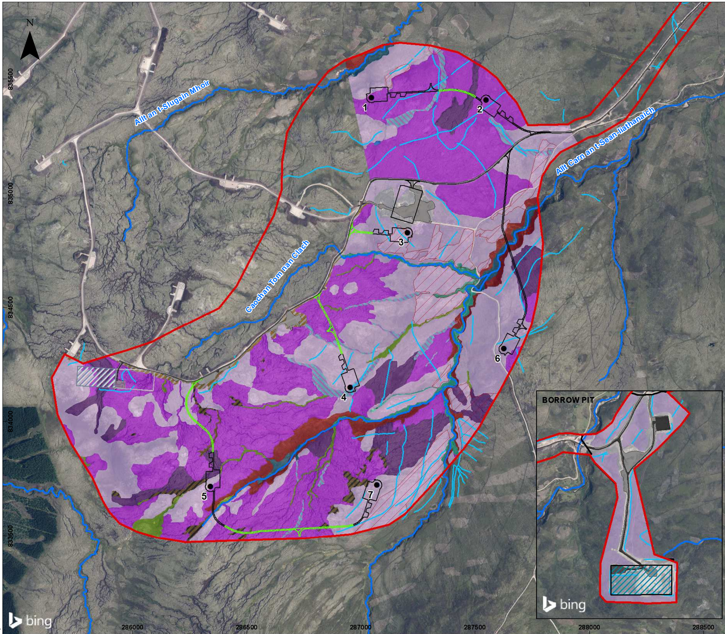
Figure 4 Geomorphology, hydrology and land-use
